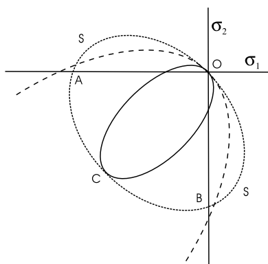
Figure 2. Elliptical yield curves used for the EVP rheology, where \sigma_1 and \sigma_2 are the principal stresses. Solid yield curve: P^* = 7.5 kN m -2 and the ratio of major to minor axes e = 2 . Dotted yield curve: P^* = 7.5 kN m -2 and e^2 = 0.5 . Curve OACBO: Truncated elliptical yield curve with e^2 = 0.5 and P^* = 7.5 kN m -2 . Dashed line: The commonly-used [Hibler and Walsh, 1982] yield curve with e = 2 and P^* = 27.5 kN m -2 .
