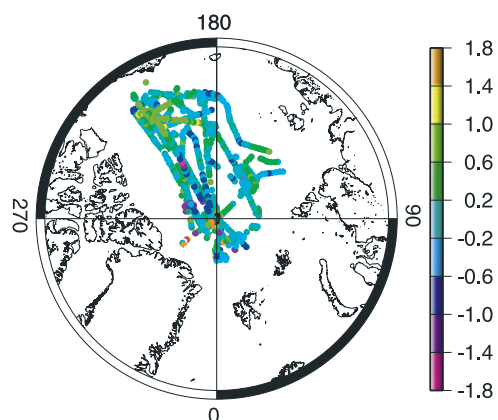
Figure 3. Modeled minus observed mean draft (m) for all cruise tracks between 1987 and 1997, for the model with e^2 = 0.5 .
