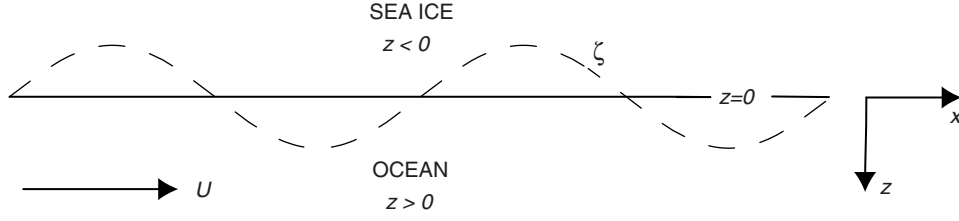
Figure 2. The geometry of the idealized sea ice–ocean system. A semi-infinite layer of sea ice ( z < 0 ) floats upon the ocean ( z > 0 ), in which there is a uniform flow U parallel to the undisturbed interface. The dashed line shows how the sea ice–ocean interface is perturbed.
